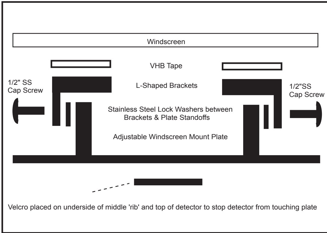
Front View of Assembly
